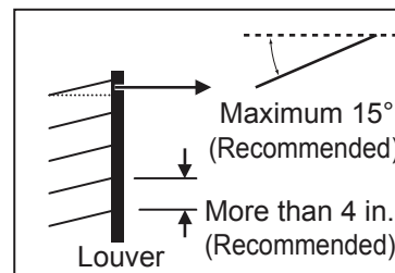
Figure 50: Louver Recommendations.
