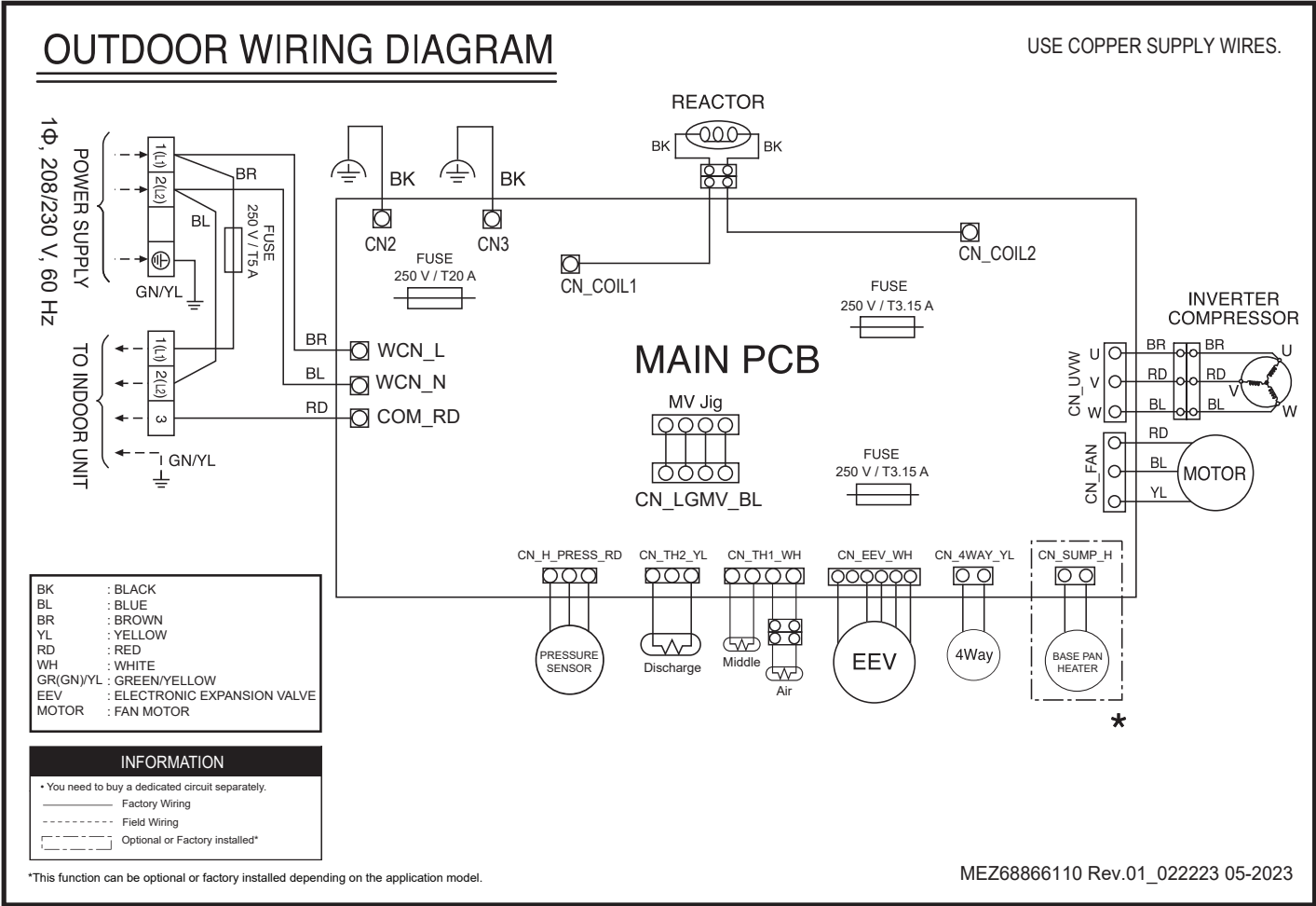
Figure 26: LUU090HV, LUU120HV Four-Way Ceiling Cassette Outdoor Unit Wiring Diagram.
