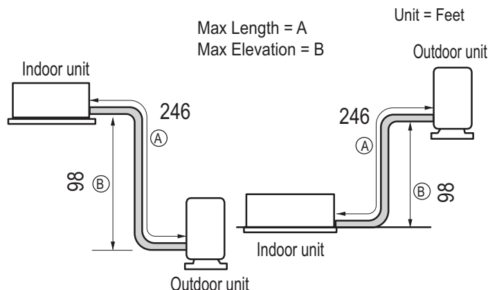
Figure 56: Typical LC369HV and LC429HV System Layout.
