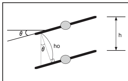
Figure 52: Open Rate by Louver Radian Formula.
