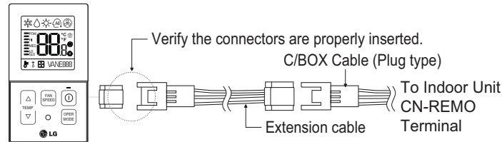
Figure 33: PZCWRC1 LG Wired Remote Extension Cable.
